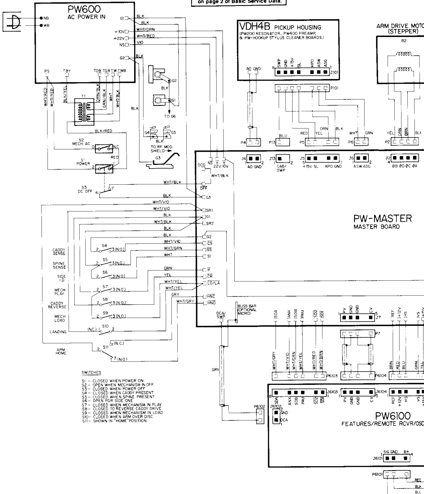
Fig. 32—Interconnect
